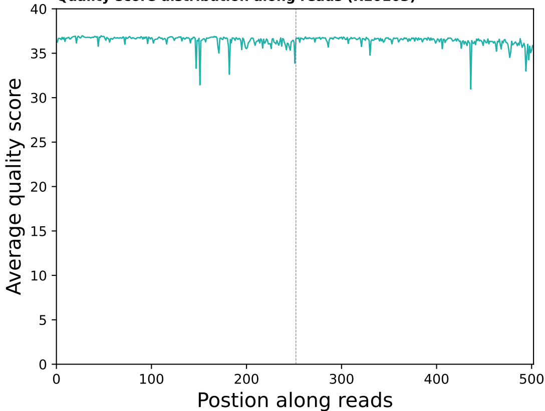
Quality score distribution along reads (R10103)
